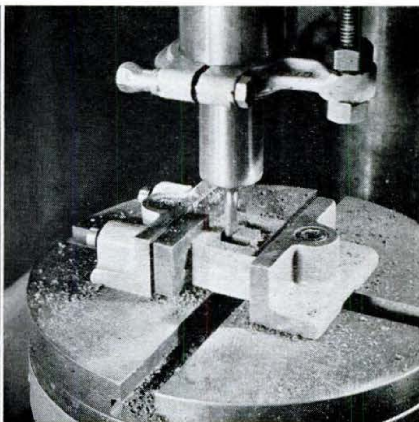
A HARDWOOD BLOCK being hollowed with a \frac{1}{4} " wood-routing bit to form a ring box. To hold such work, a special vise may be purchased to fit the T slots in the table. Jaws can be locked anywhere along the table slots.
